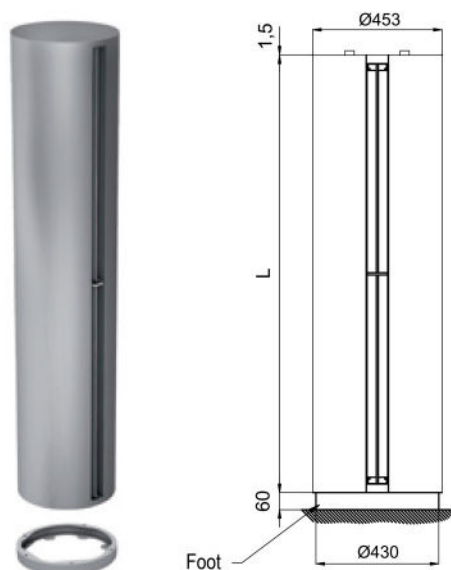
Vertical installation
