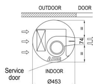
Standard installation (vertical left side)
