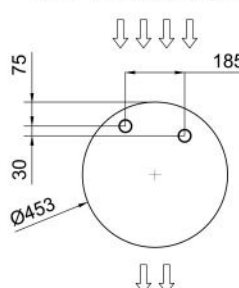
Floor fixing points with foot
