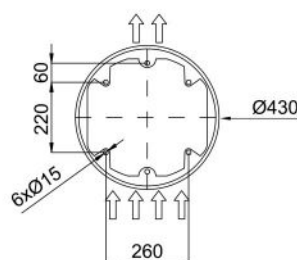
Floor fixing points with foot
