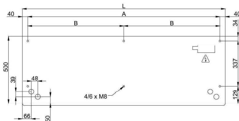
WINDBOX M,ECM,G,ECG Air Curtain Installation Configurations with False Ceiling Kits
