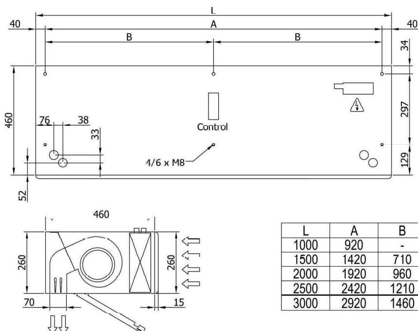
WINDBOX M,ECM,G,ECG Air Curtain Installation Configurations with False Ceiling Kits
