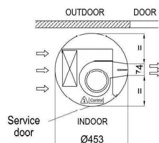
Standard installation (vertical left side)
