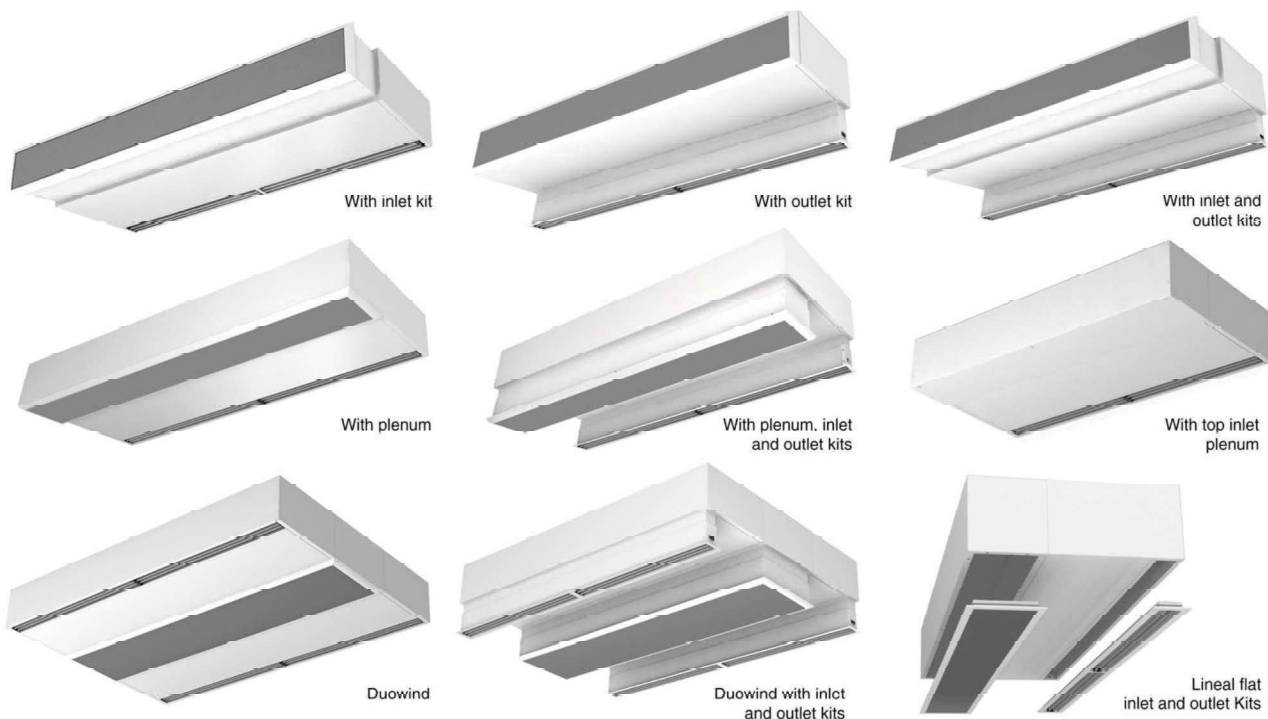
WINDBOX M,ECM,G,ECG Air Curtain Installation Configurations with False Ceiling Kits
